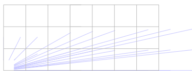
full space-time attention every patch ↔ every patch (all frames)
